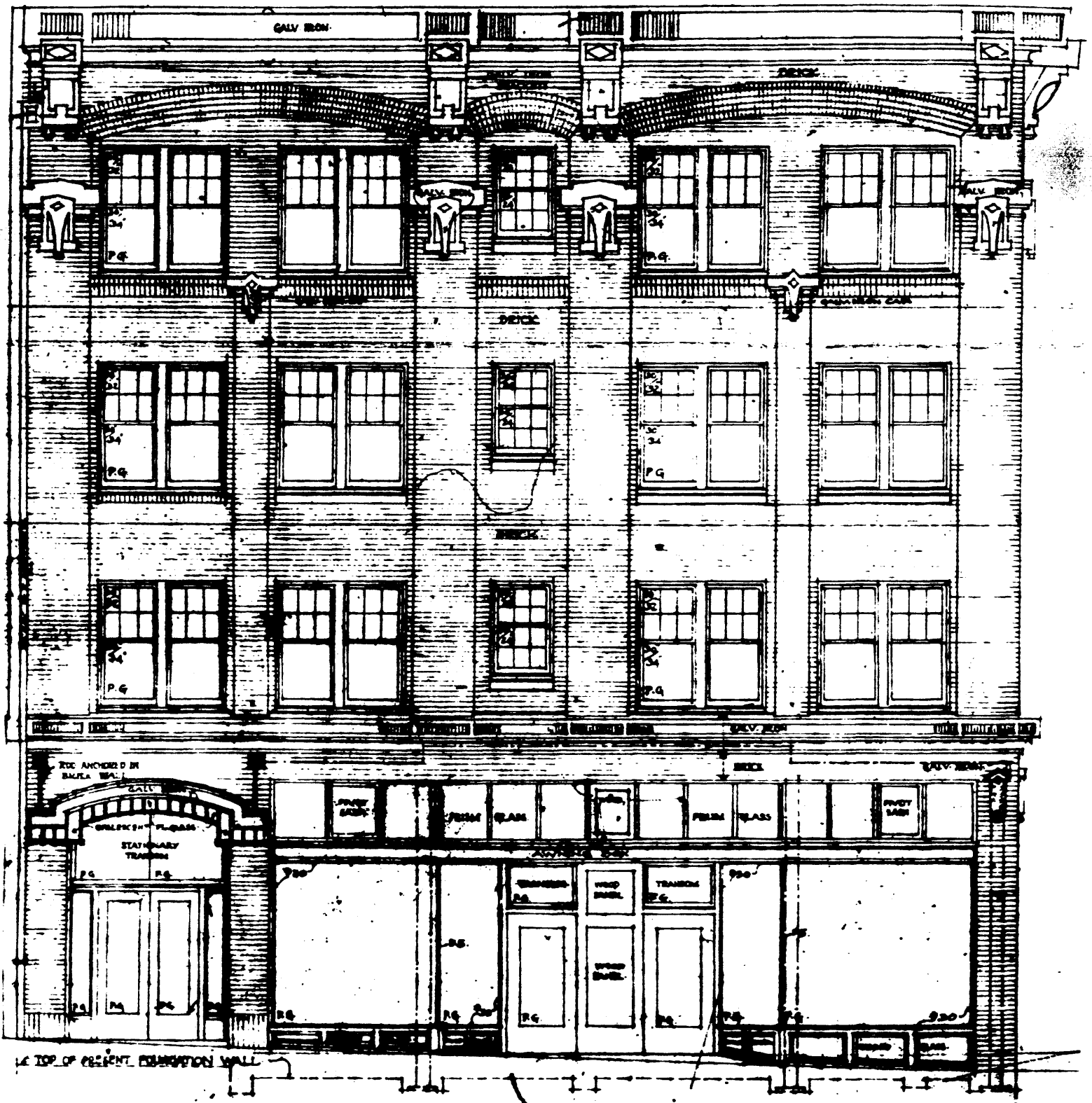
- 12 th STREET ELEVATION - SCALE \frac{1}{4} " = 1'-0"
