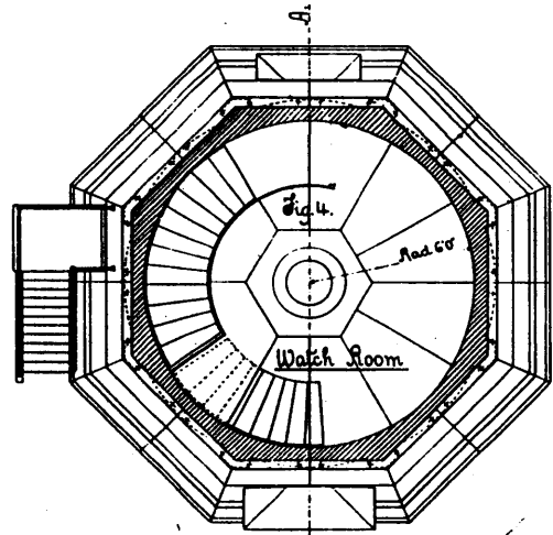
Sectional Plan C.C.
