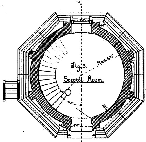
Sectional Plan B.B.
