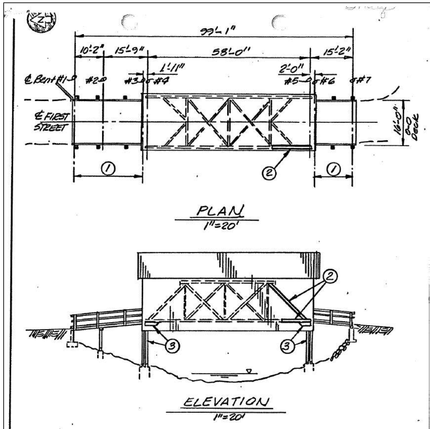
Figure 6. Engineering Plans (pre-relocation)
