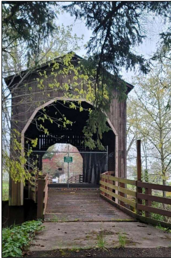
Photograph 7 of 9: OR_DouglasCounty_PassCreekCoveredBridge_0007 South portal of Pass Creek Covered Bridge and replacement approach span, camera facing north.
