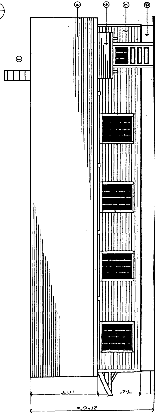
SOUTH ELEVATION MAIN HATCHERY BUILDING
