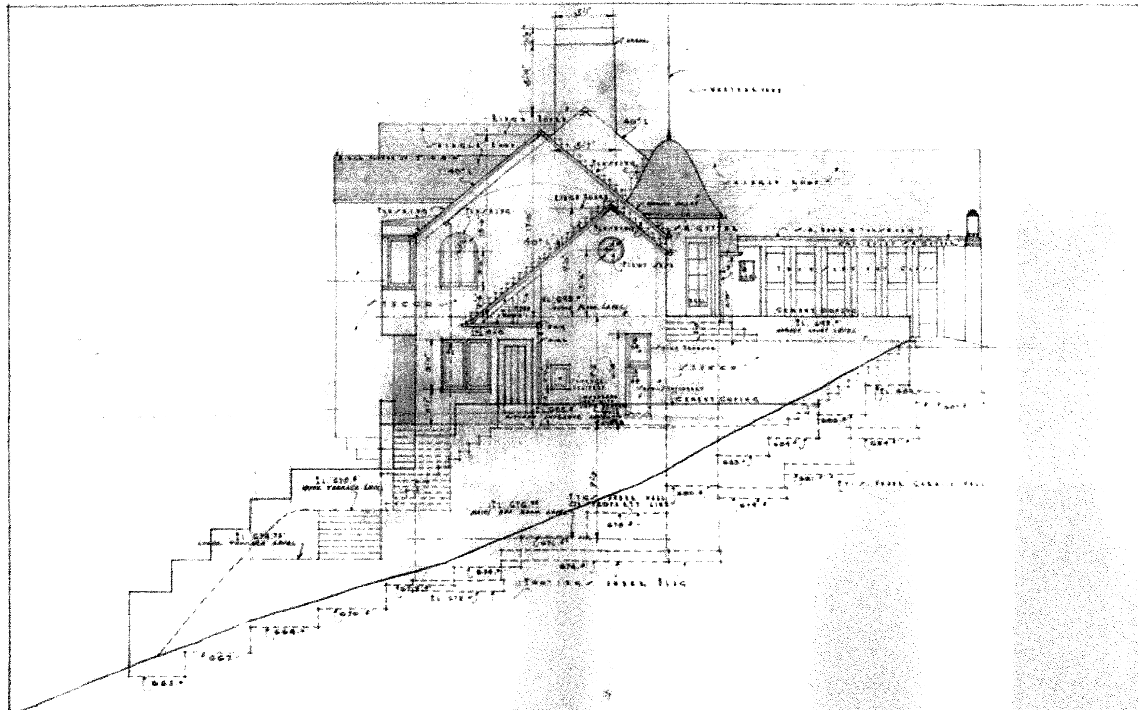
· NORTH-WEST ELEVATION · SCALE 1/4" = 1'-0" · HOUSE FOR V. JORGENSEN · S. O. · PORTLAND ORE ·
