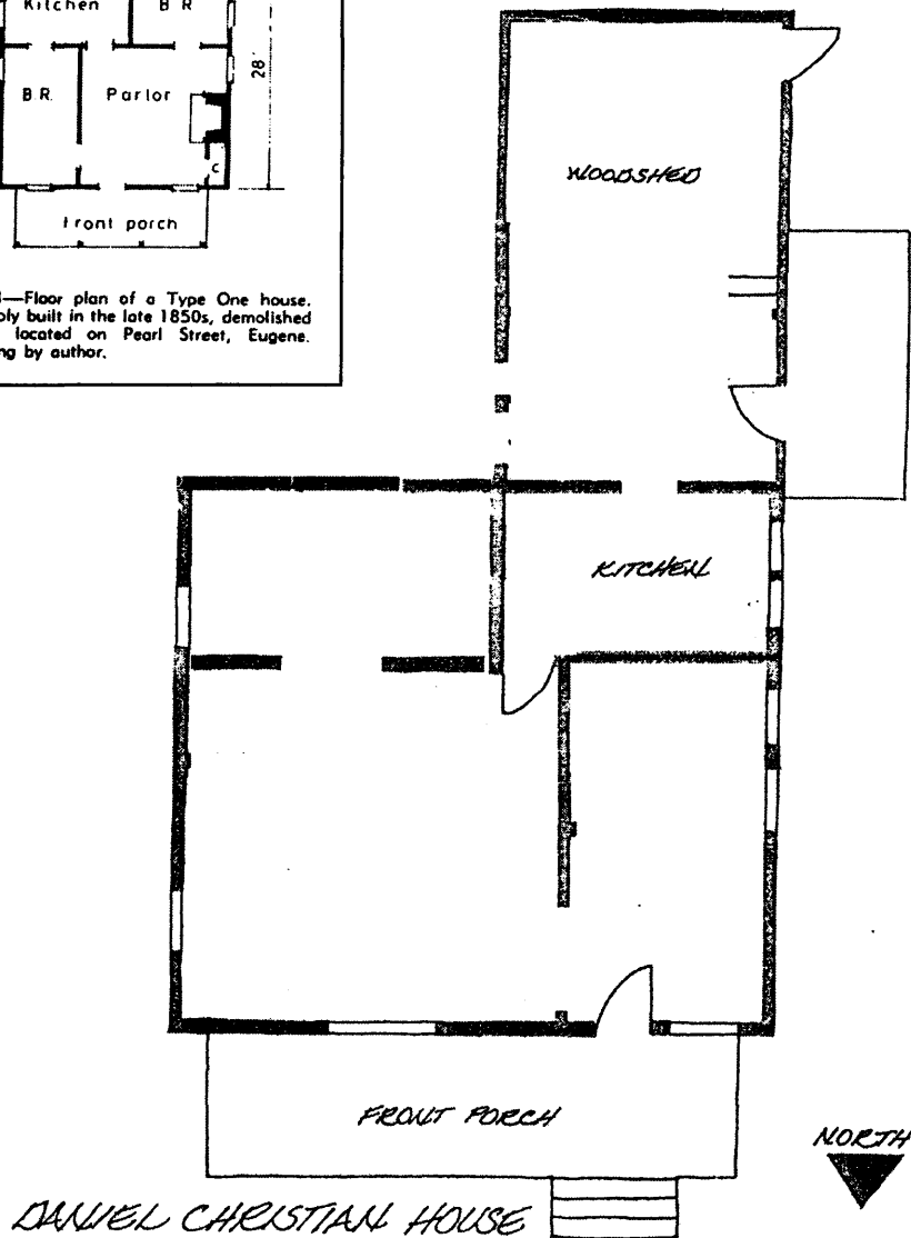
Figure. 18. Possible original configuration of first floor plan based on substructure arrangement and comparison to similar house described by Dole. Inset: Drawing from Dole's article "Farmhouse & Barn in Early Lane County" showing Type 1 house floor plan.
